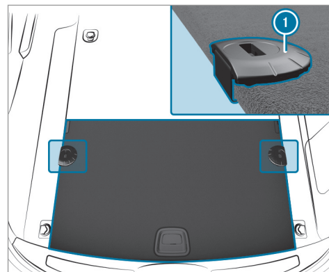
① Telescopic rod with mounting elements and holders
